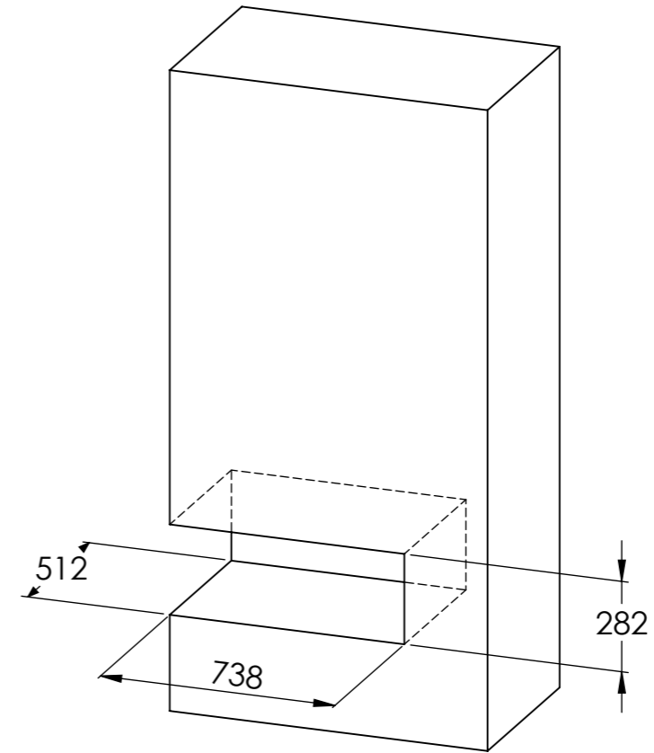
Prestige BL Log store without frame
