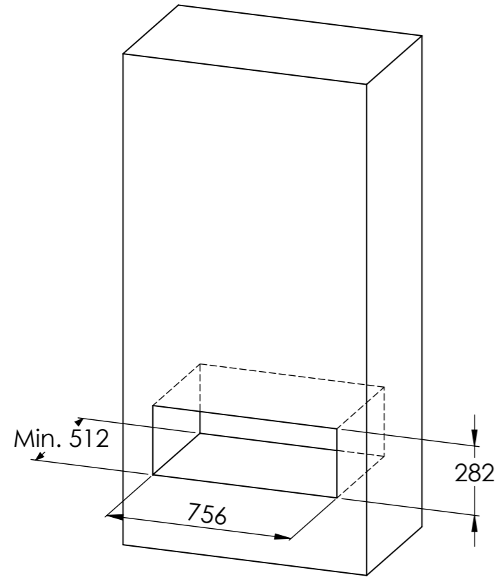
Prestige A Log store without frame
