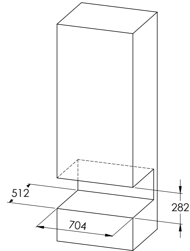
Prestige C Log store without frame
