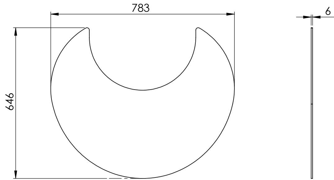
Scan-Line 900 (0021-014465)
