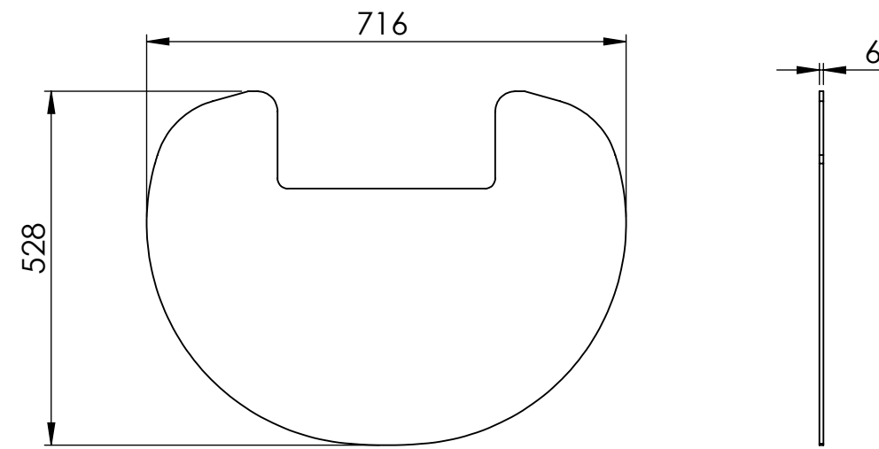
Scan-Line 7B (0021-014466)
