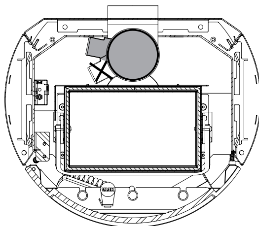
HAC motor position.
